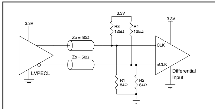
Figure 4C. CLK/nCLK Input Driven by a 3.3V LVPECL Driver
