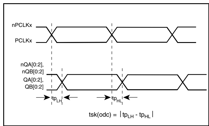
Output Duty Cycle Skew
