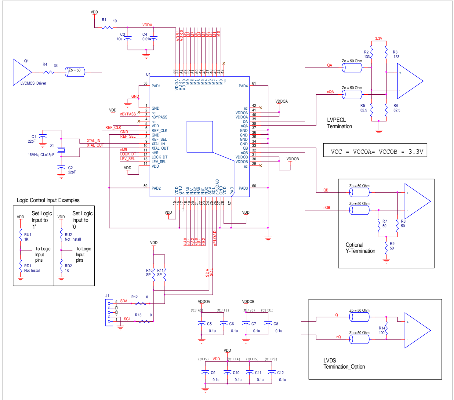
Figure 7. ICS844S42I Schematic Example
