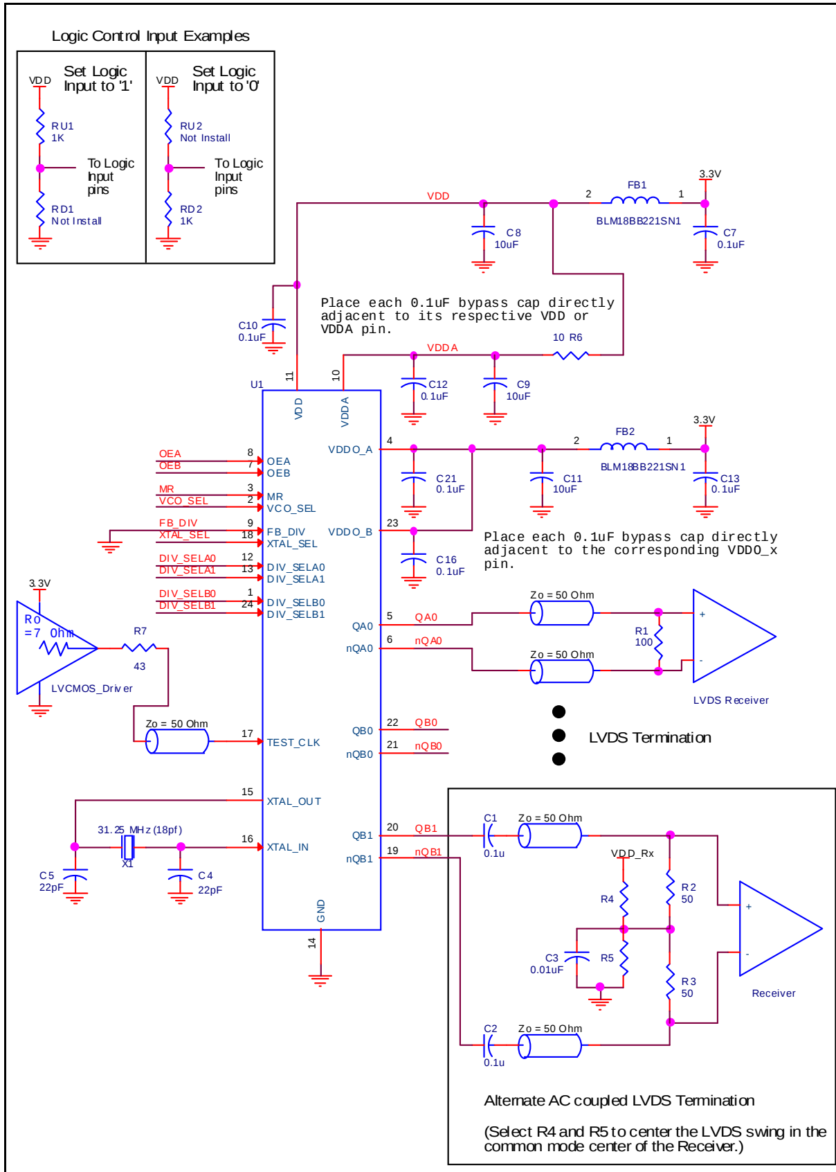
Figure 3. 844003 Application Schematic
