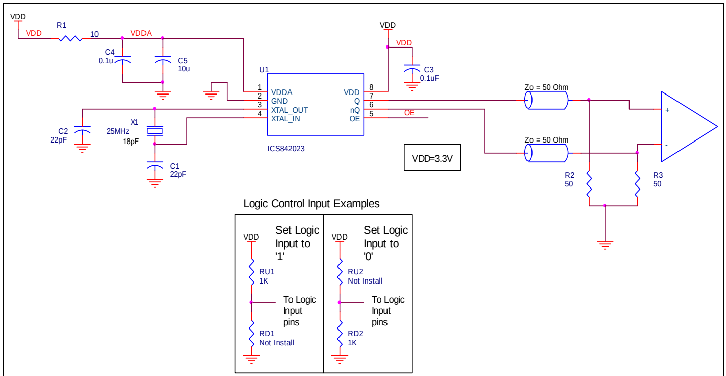
Figure 5. 842023 Schematic Example
