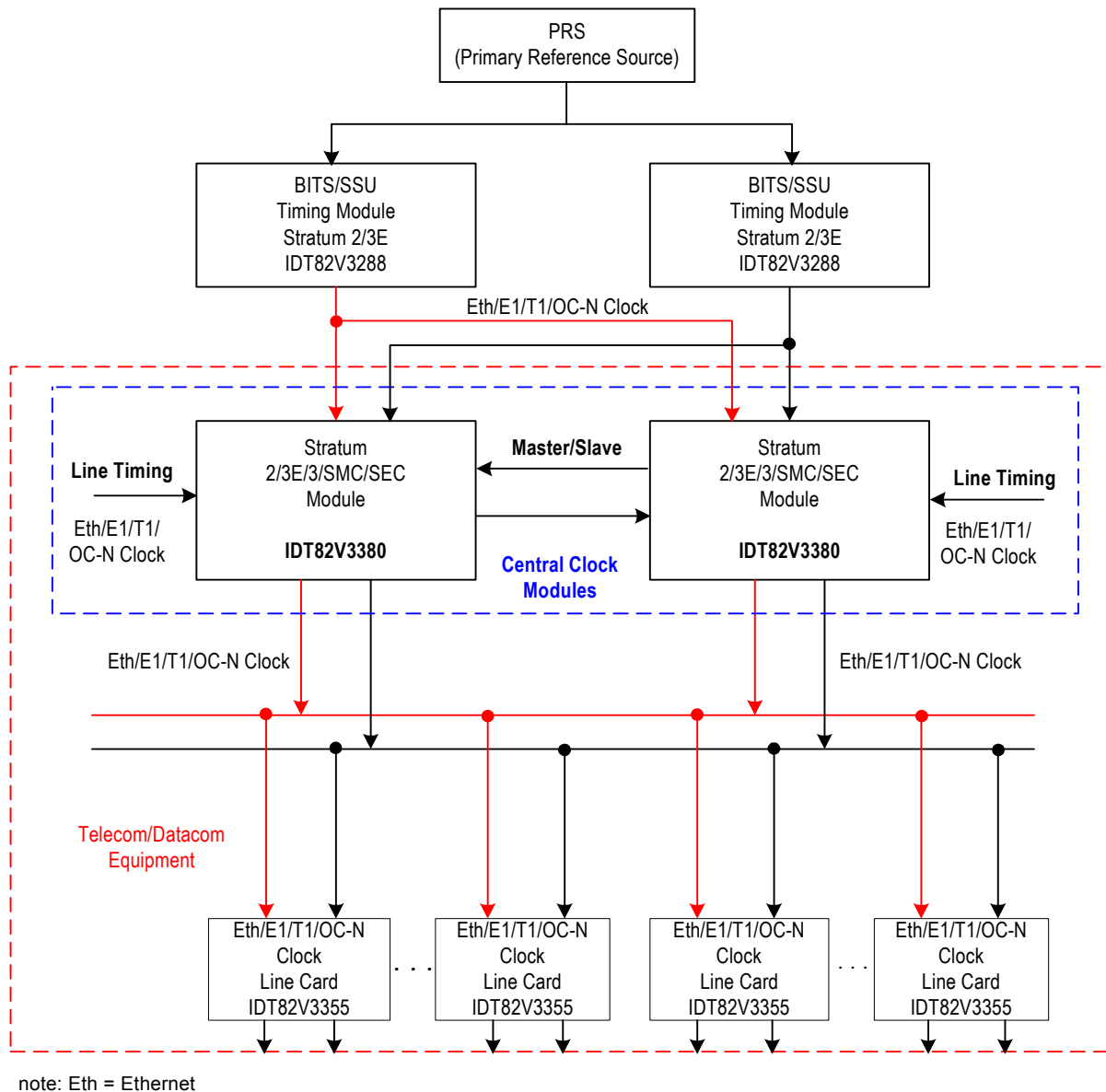
Figure 15. Typical Application
