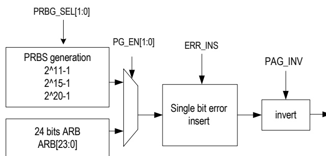
Figure-23 Pattern Generation (2)
