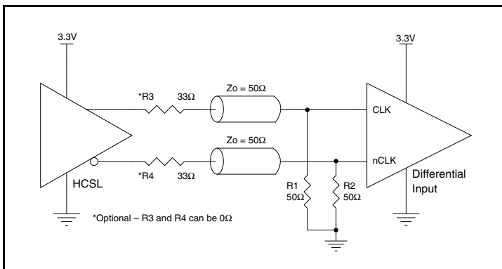
Figure 2E. CLK/nCLK Input Driven by an HCSL Driver
