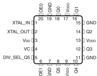
ICS81006I 20-Lead VFQFN 4mm x 4mm x 0.925 package body K Package Top View
