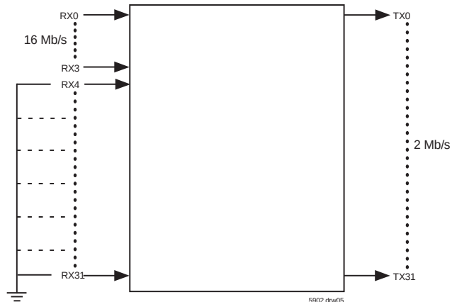
Figure 4. Mux/Demux Mode
