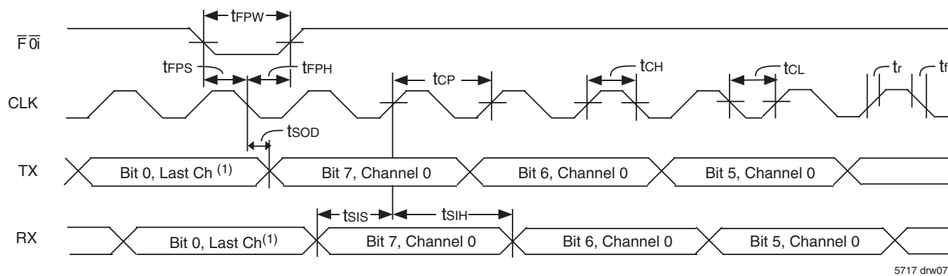
Figure 7. ST-BUS® Timing
