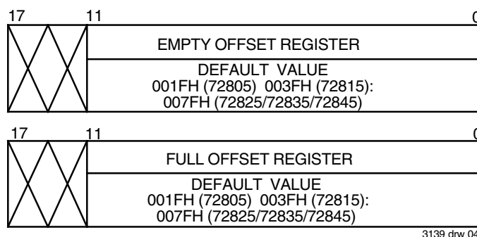
Figure 2. Writing to Offset Registers
