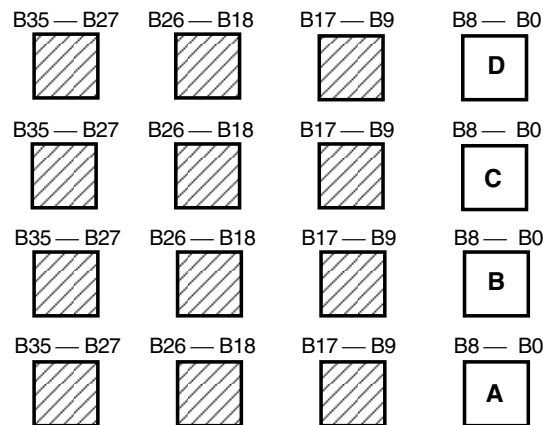
Figure 2. Bus sizing
