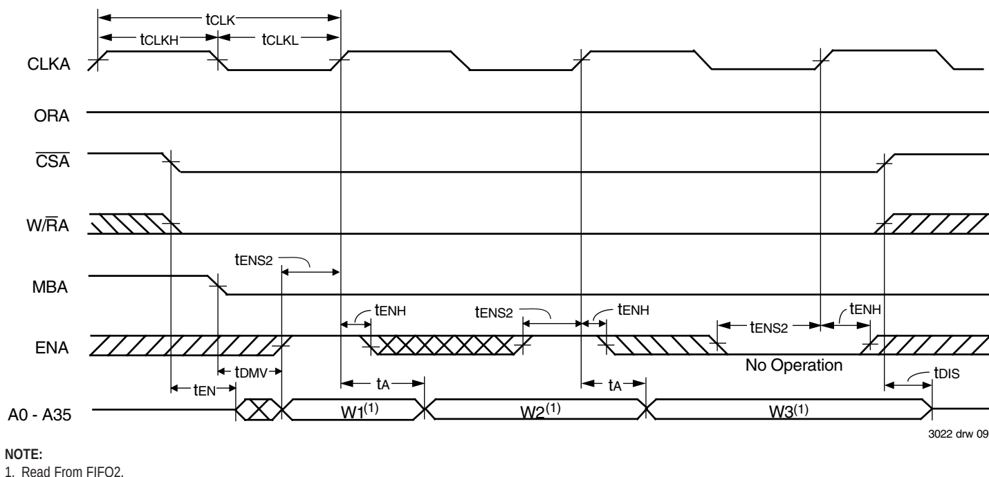
Figure 7. Port A Read Cycle Timing for FIFO2
