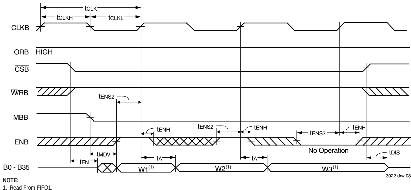
Figure 6. Port B Read Cycle Timing for FIFO1
