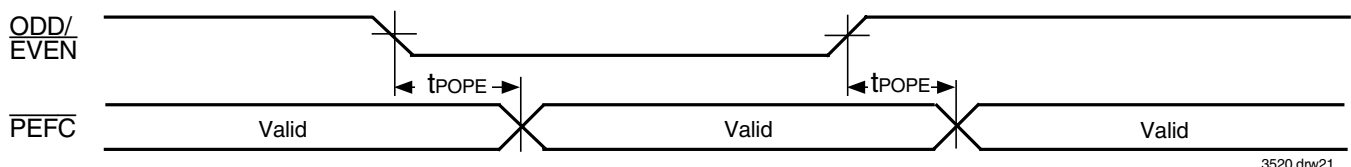
Figure 21. ODD/ \overline{EVEN} to \overline{PEFC} Timing
