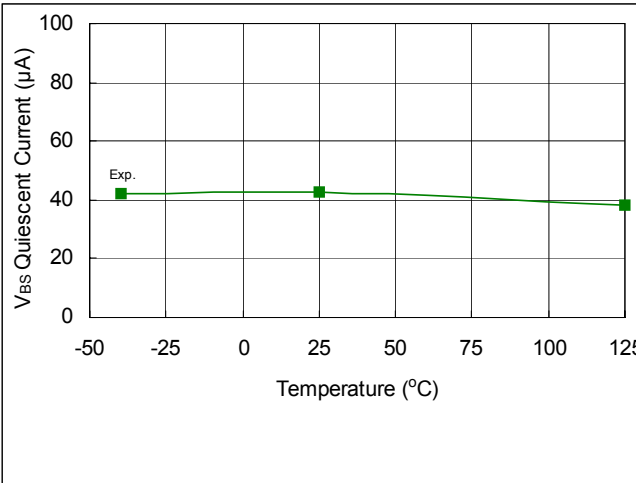
Fig. 29 V BS Quiescent Supply Current vs. Temperature
