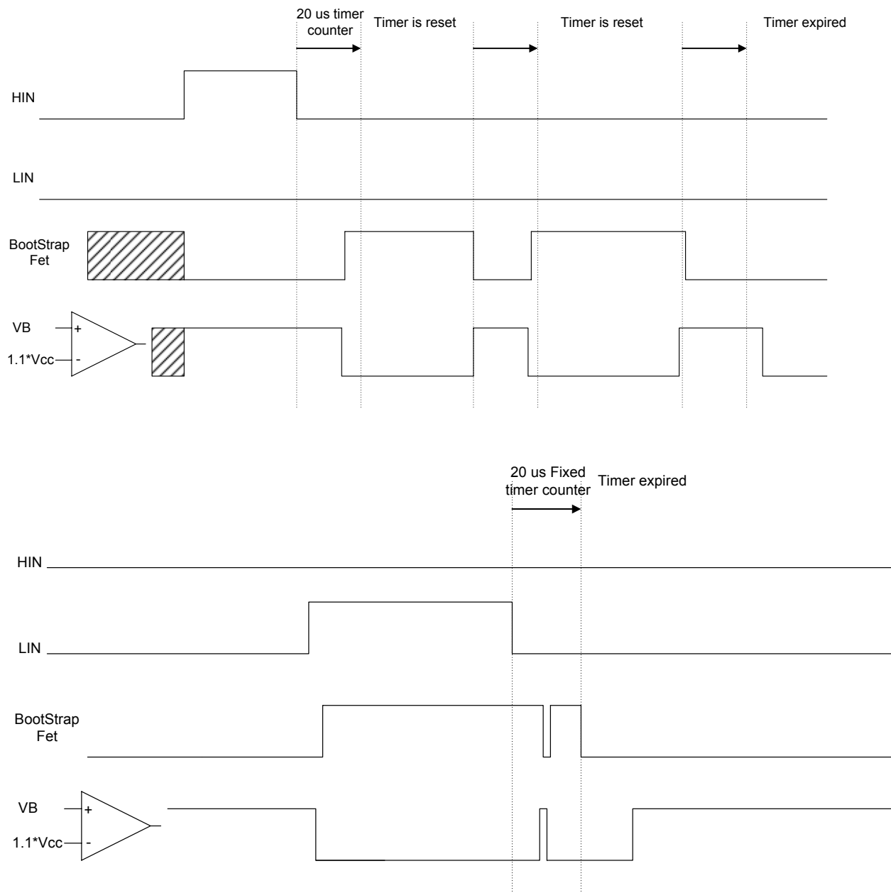
Figure 9: BootFET timing diagram
