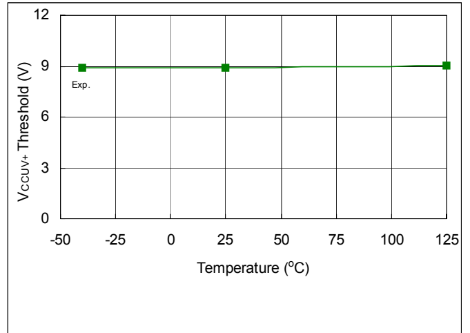
Fig. 38. V_{CCUV+} Threshold vs. Temperature
