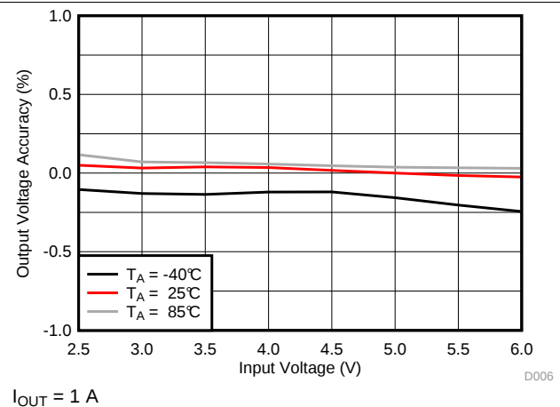
Figure 17. Line Regulation
