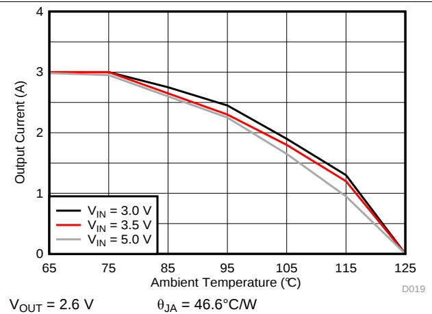
Figure 15. Thermal Derating
