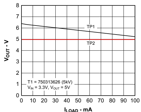
Figure 6-25. Output Voltage vs Load Current
