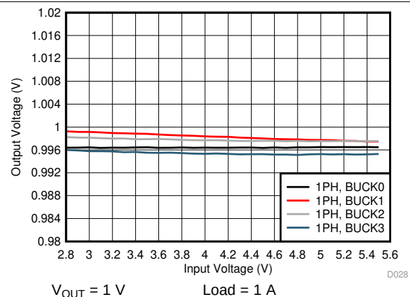
Figure 72. Output Voltage vs Input Voltage in PWM Mode
