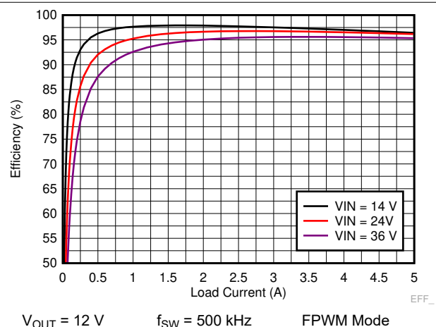
Figure 9-20. LM73605-Q1 Efficiency
