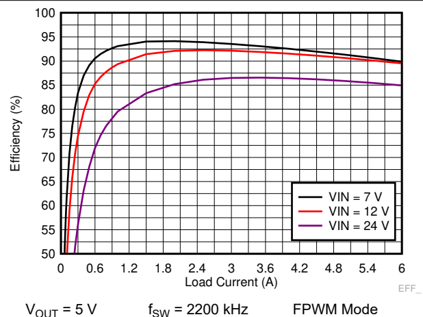
Figure 9-18. LM73606-Q1 Efficiency
