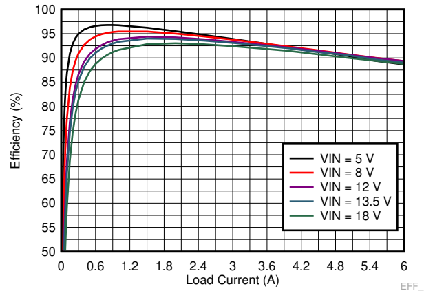
Figure 9-4. LM73606-Q1 Efficiency
