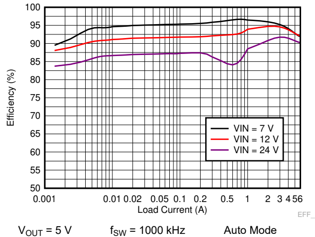
Figure 9-15. LM73606-Q1 Efficiency
