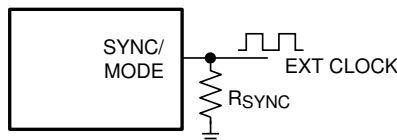
Figure 8-13. Frequency Synchronization
