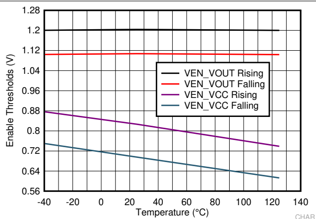
Figure 7-8. Enable Thresholds
