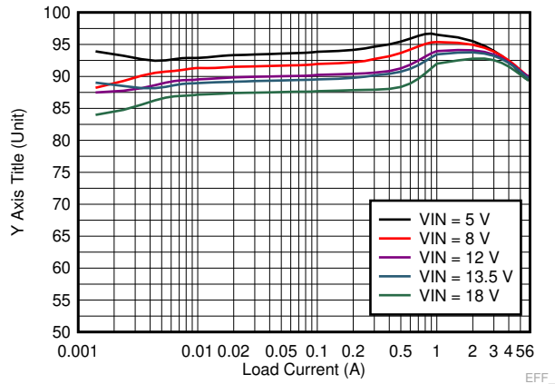
Figure 9-3. LM73606-Q1 Efficiency
