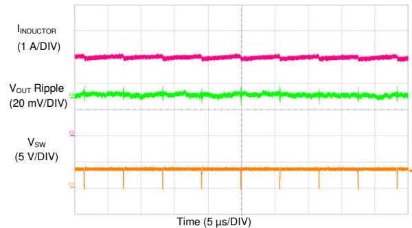
Figure 9-48. LM73606-Q1 Switching Waveform and V_{OUT} Ripple
