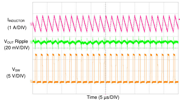
Figure 9-46. LM73606-Q1 Switching Waveform and V_{OUT} Ripple
