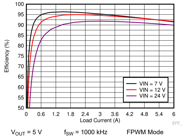
Figure 9-16. LM73606-Q1 Efficiency
