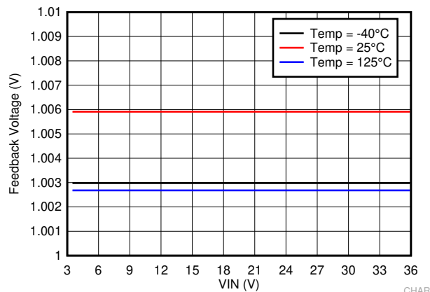
Figure 7-3. Feedback Voltage
