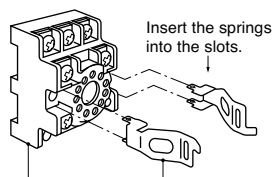
Socket SR3P-05A Hold-Down Spring (optional) SFA-203 (2 pcs/set)
