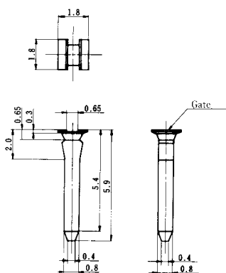
HIF3-GPIN(A)
