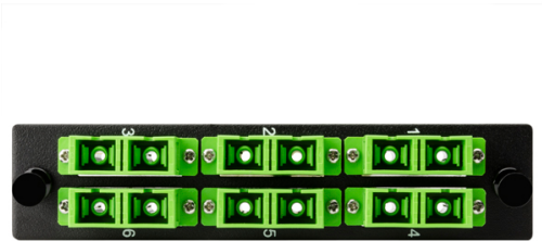
Fiber Adapter Panel Preloaded with 6 Duplex SC SMA, Green, 1/pkg
