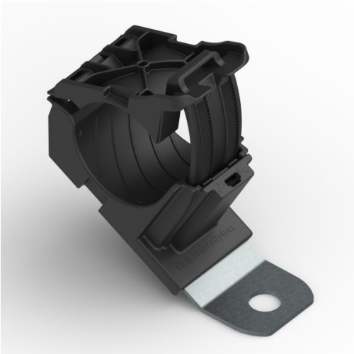
Ratchet P-Clamp, 0.76 - 1.42" Bundle Dia, 30° Short, .41" Hole Dia, PA66HIRHSUV/SS304, Black, 160/ctn
