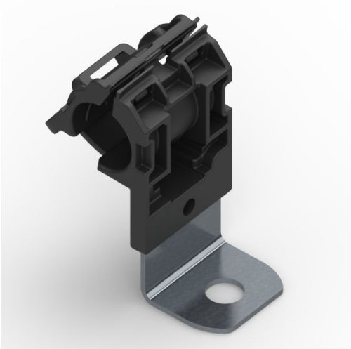
Ratchet P-Clamp, 0.52" - 0.77" Bundle Dia, 90° Short, .51" Hole Dia, PA66HIRHSUV/SS304, Black, 280/ctn
