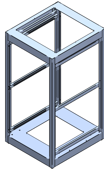
ISOMETRIC
