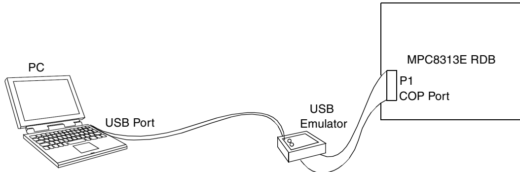
Figure 18. Connecting MPC8313E-RDB to a USB Emulator
