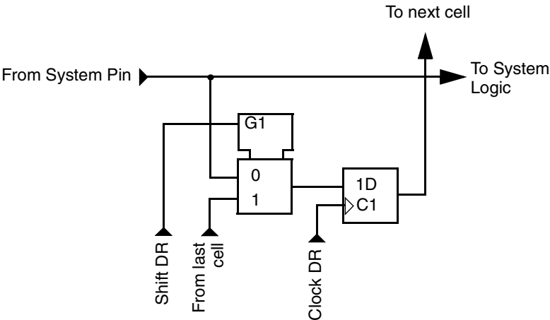
Figure 7 Observe-Only Cell
