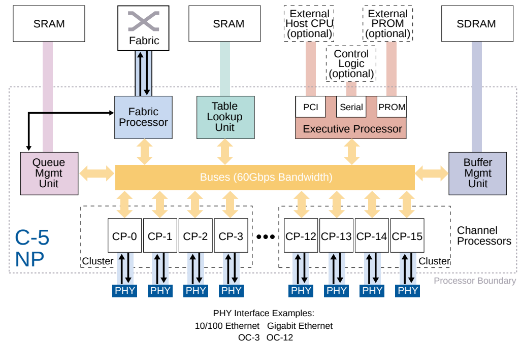
Figure 1 C-5 Network Processor Block Diagram
