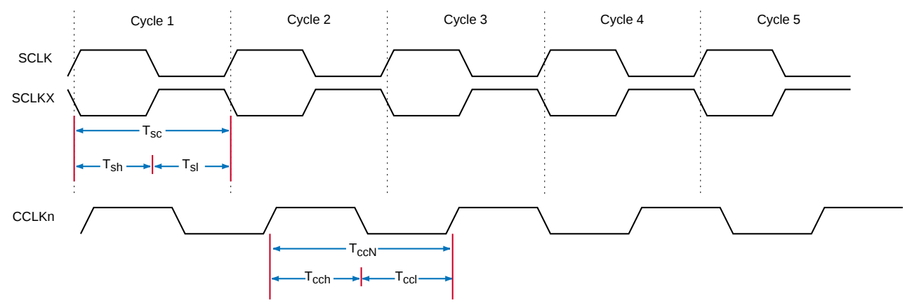
Figure 12 System Clock Timing Diagram
