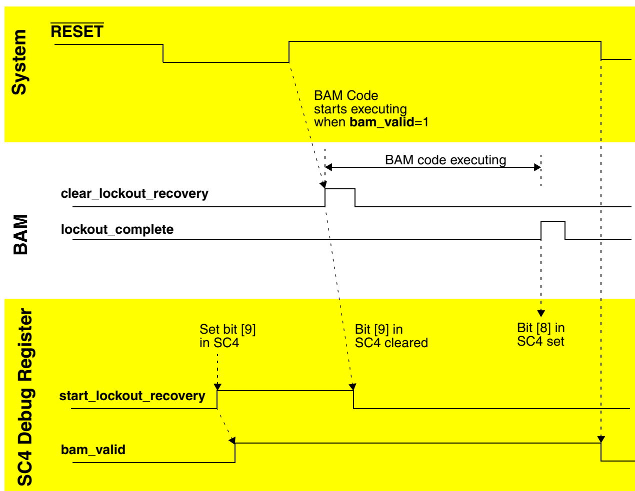
Figure 20-1. BAM Sequence
