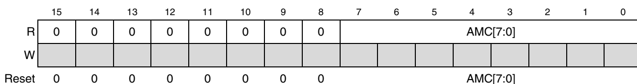
Figure 13-3. AXBS Master Configuration (AMC) Register
