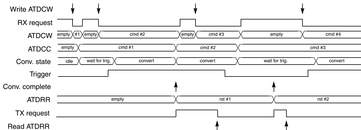
Figure 33-32. Conversion Procedure for Example 4
