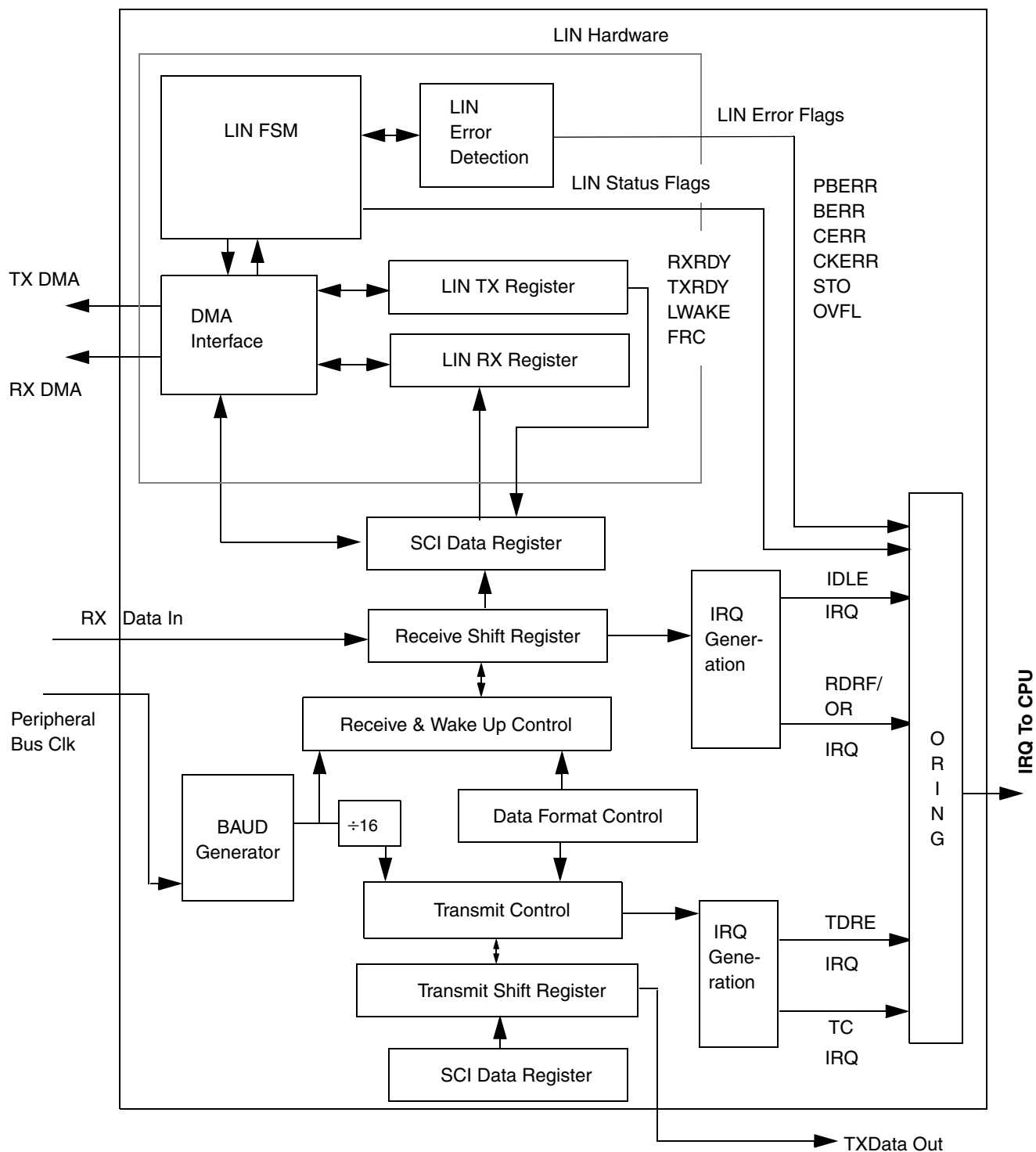
Figure 31-1. eSCI Block Diagram
