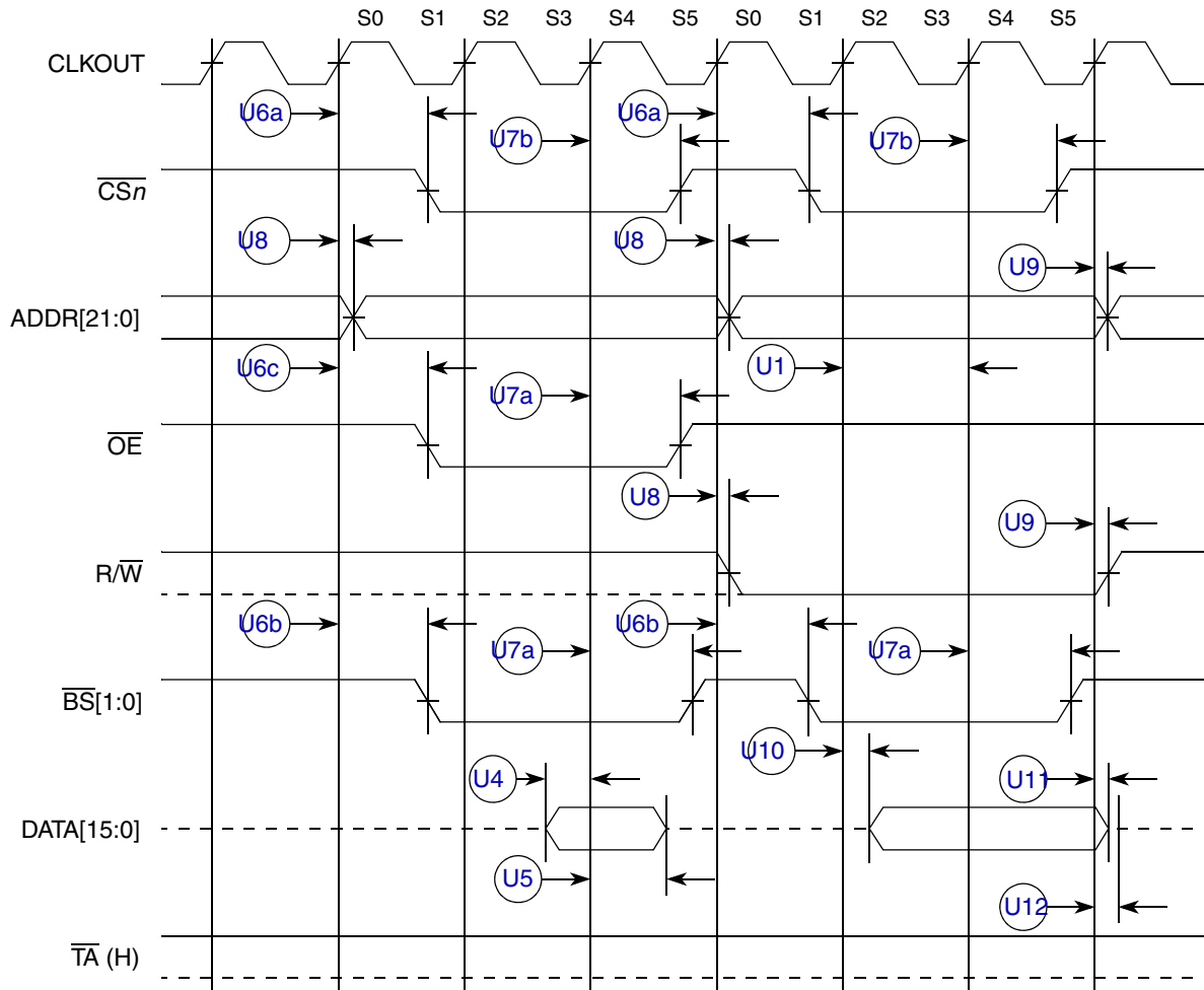
Figure A-11. Read/Write (Internally Terminated) Bus Timing
