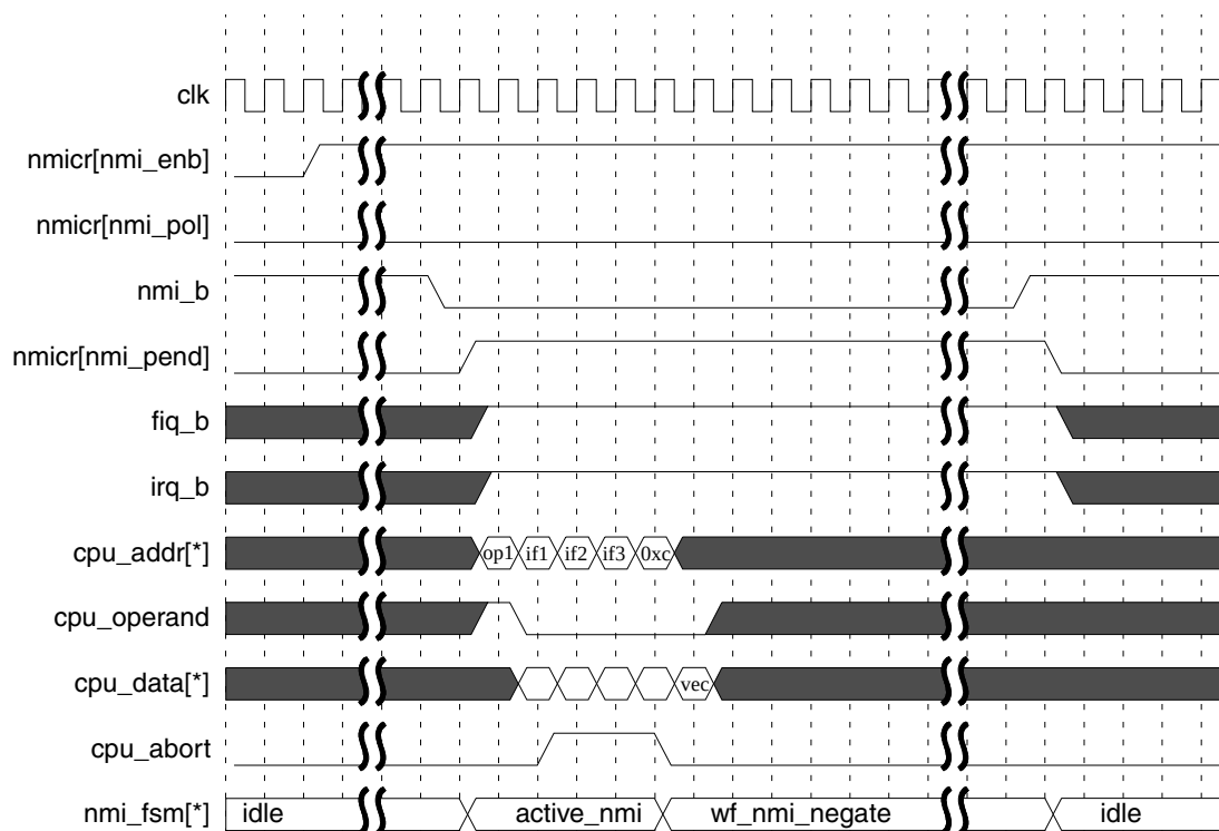
Figure 13-14. Non-Maskable Interrupt Operation Timing
