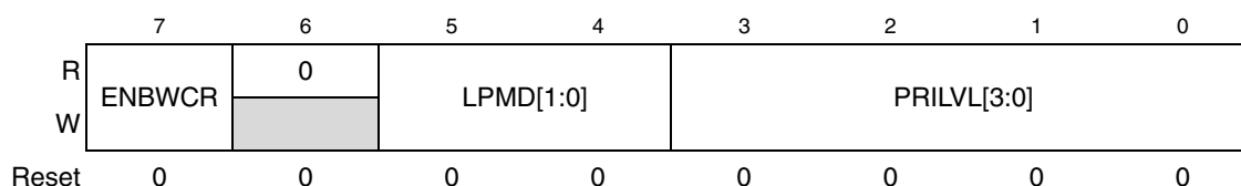
Figure 13-7. Miscellaneous Wakeup Control (MWCR) Register
