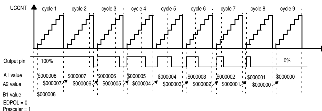
Figure 32-42. OPWFMB Mode from 100% to 0% Duty Cycle
