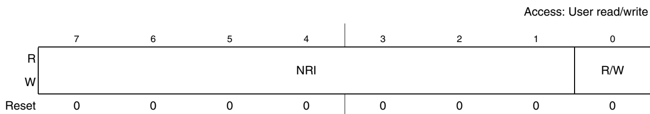
Figure 11-23. JTAG DR for Nexus Register Access
