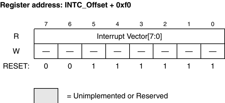
Figure 14-12. FIQ Interrupt Acknowledge Register (FIQIACK)
