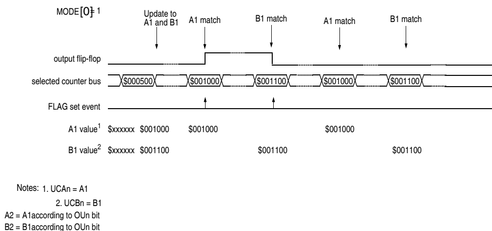
Figure 32-22. Double Action Output Compare with FLAG set on both matches
