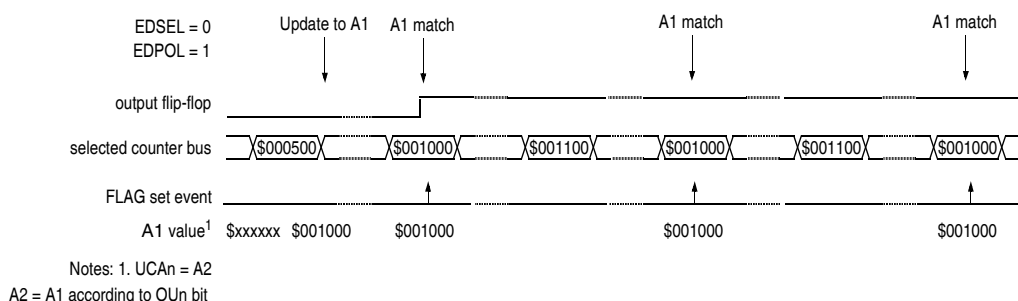
Figure 32-15. SAOC example with EDPOL value being transferred to the output flip-flop
