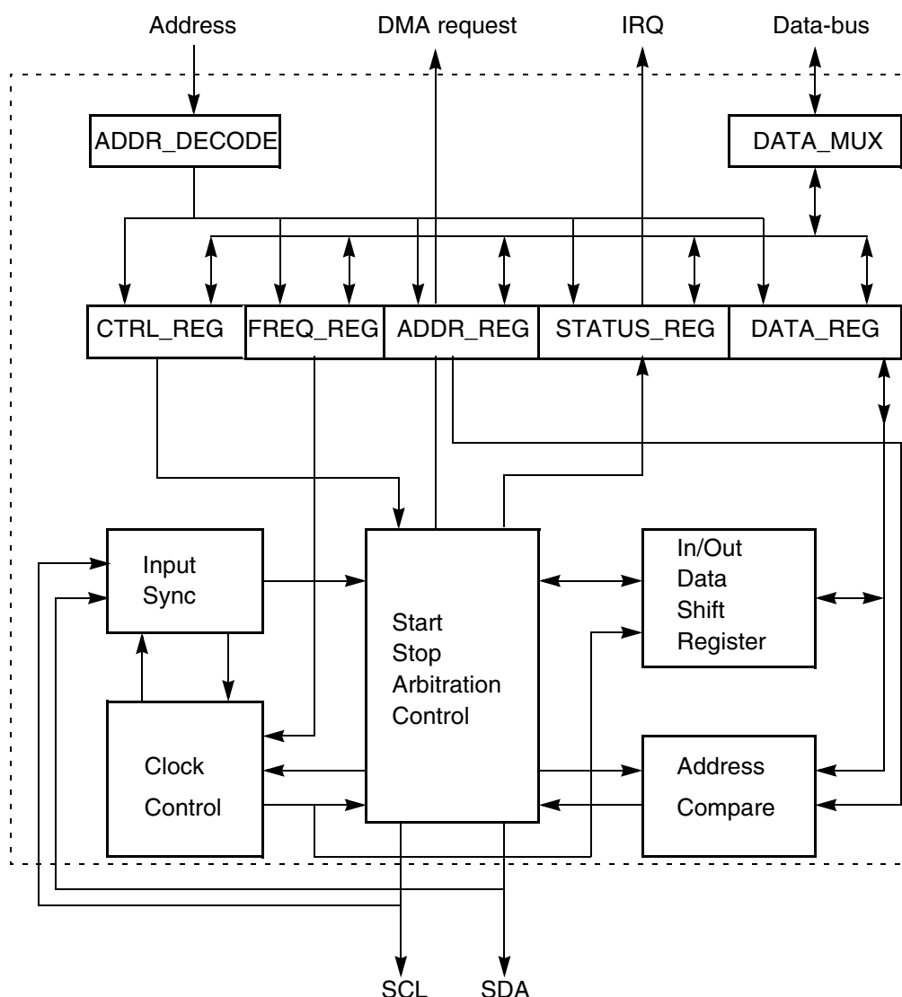
Figure 29-2. I²C Module DMA Interface Block Diagram
