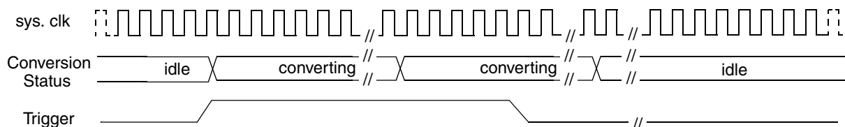
Figure 33-33. ATD Level-Based Minimum Trigger
