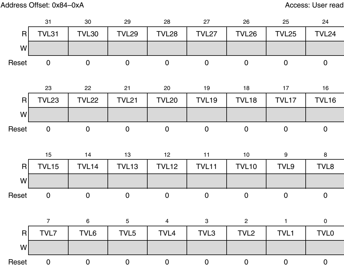
Figure 26-5. PIT CurrentTimer Values (TVAL1–10)
