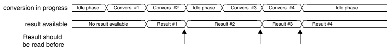
Figure 33-19. Command vs. Result Timing
