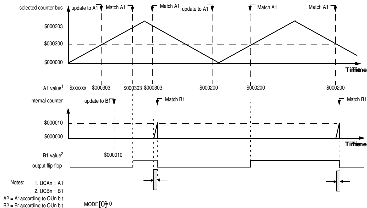
Figure 32-44. Output PWM with trailing dead time insertion
