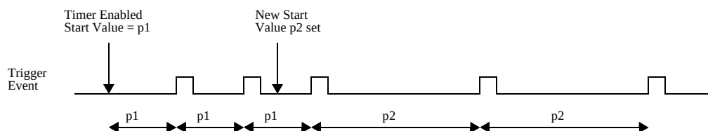
Figure 26-13. Dynamically Setting a New Load Value
