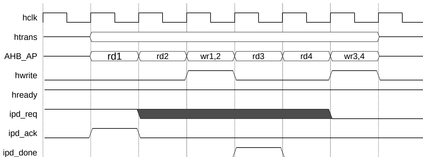
Figure 12-25. ipd_req removal
