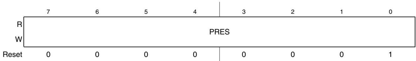
Figure 33-4. ATD Prescaler Register (ATDPRE)
