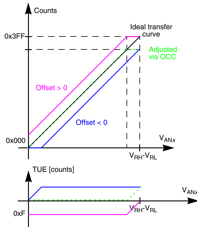
Figure 33-26. Offset Error Compensated via OCC
