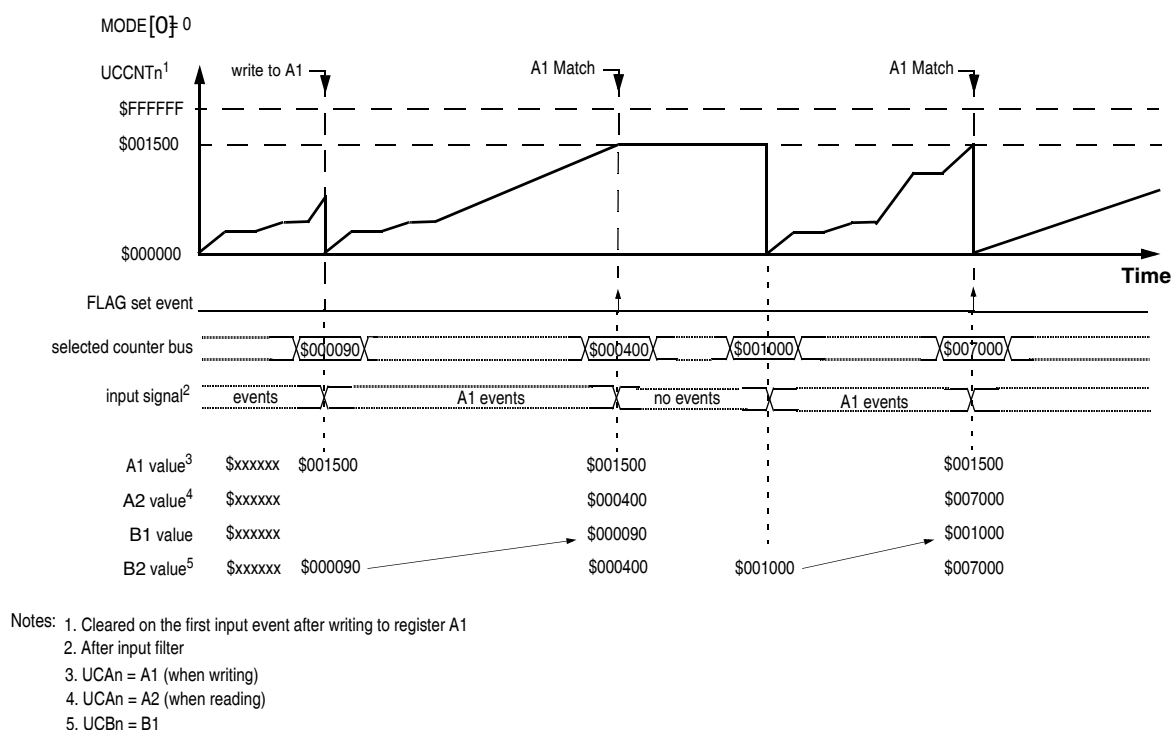
Figure 32-23. Pulse/Edge Accumulation continuous mode example
