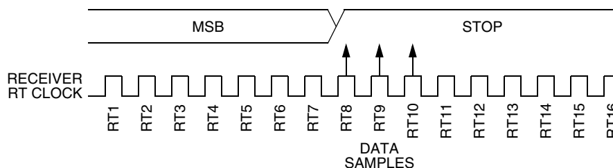
Figure 31-34. Slow Data
