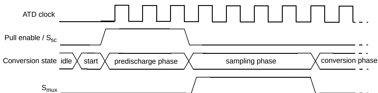
Figure 33-22. Predischarge Timing
