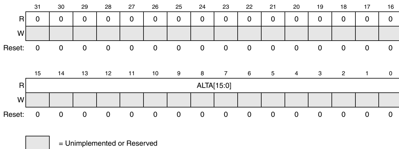
Figure 32-12. eMIOS Alternate A register (ALTAn)
