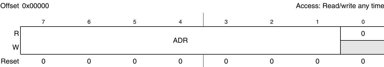
Figure 29-4. I 2 C Bus Address Register (IBAD)
