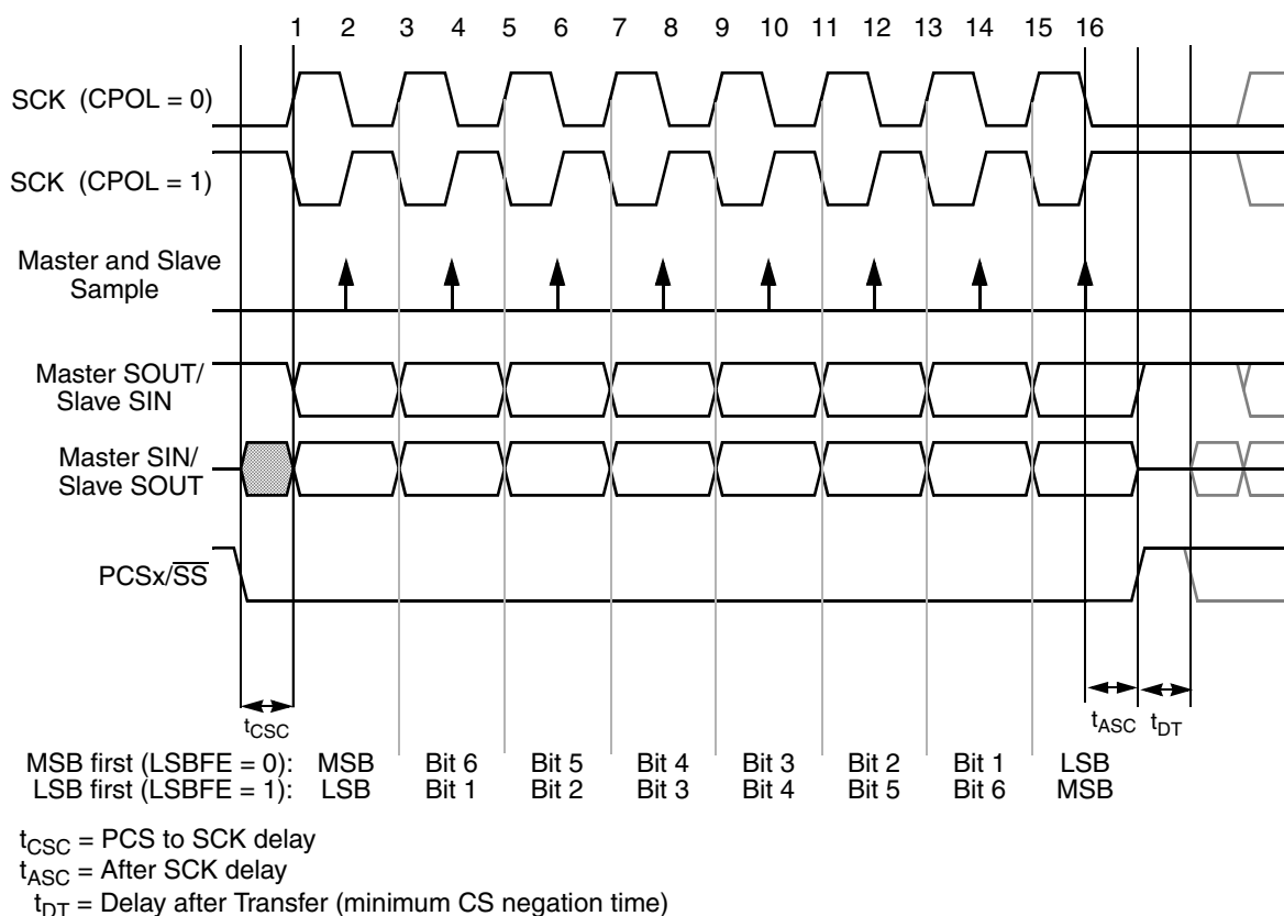
Figure 30-17. DSPI Transfer Timing Diagram (MTFE=0, CPHA=1, FMSZ=8)
