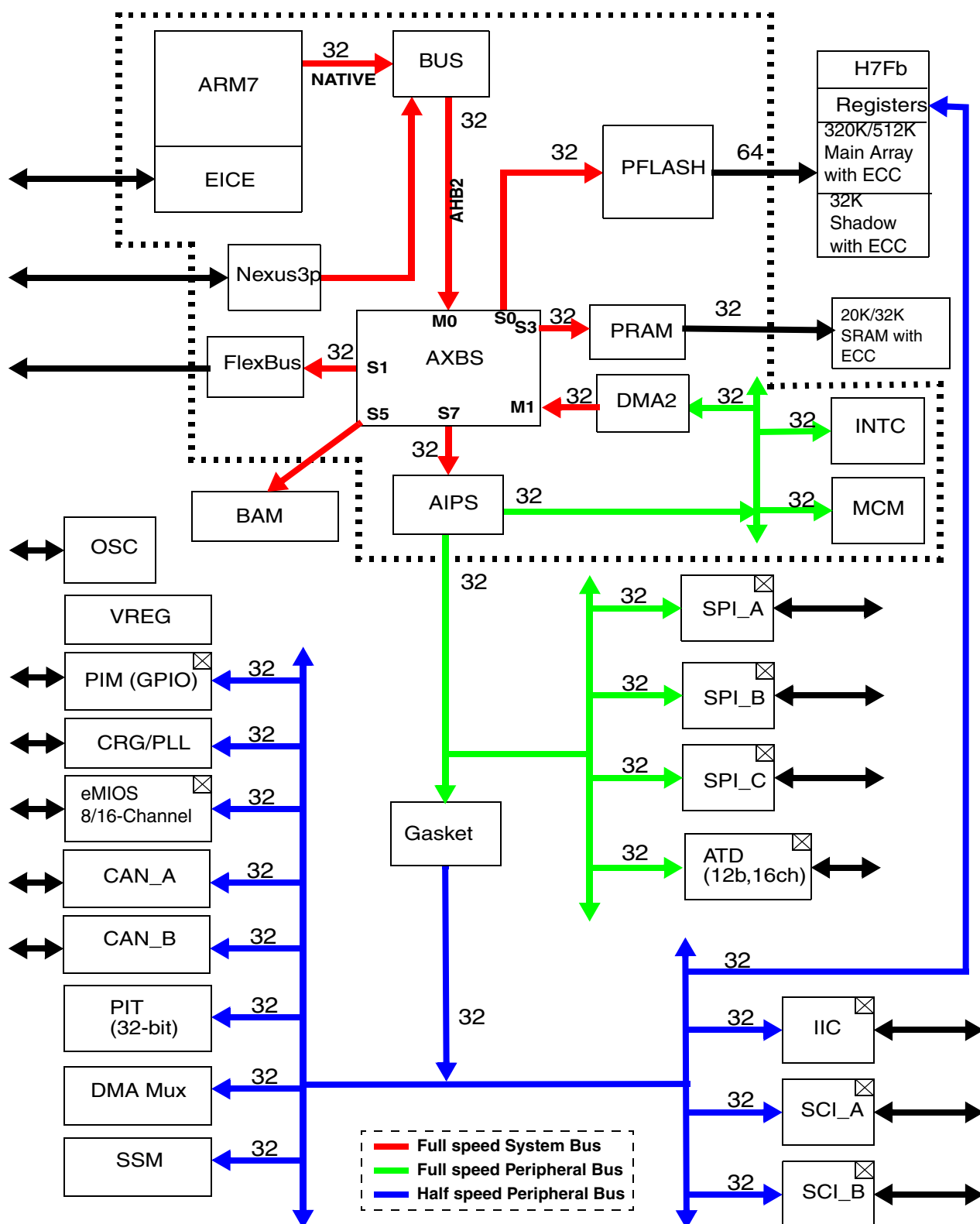
Figure 1-2. MAC72xx Architecture Overview
