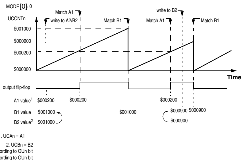
Figure 32-36. OPWFM with immediate update
