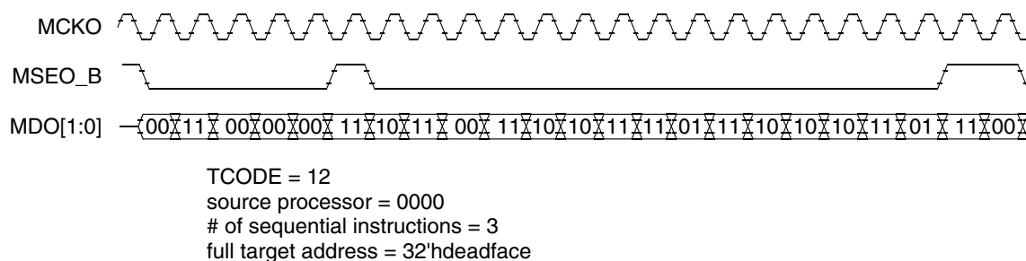
Figure 11-38. Program Trace – Indirect Branch w/ Sync. Message (Traditional)
