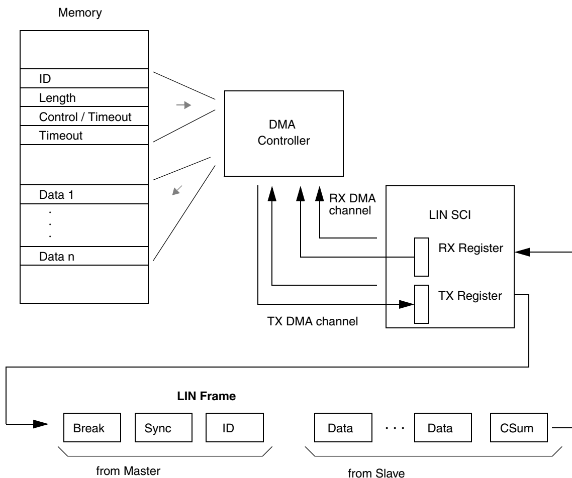
Figure 31-40. DMA transfer of a RX frame
