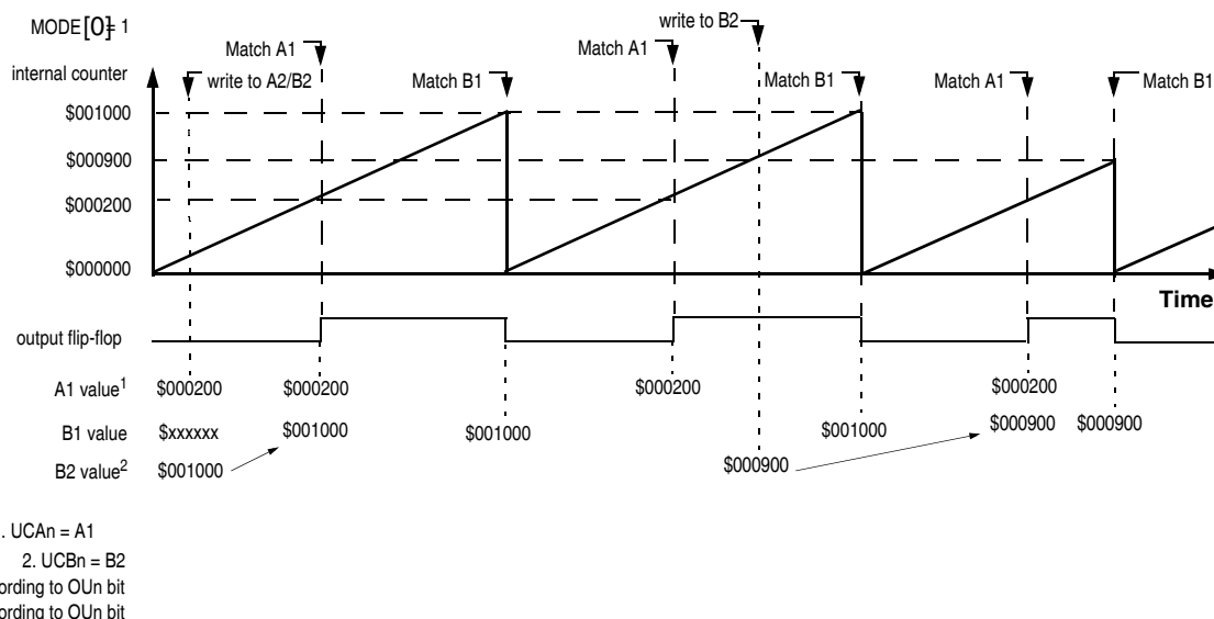
Figure 32-37. OPWFM with next period update
