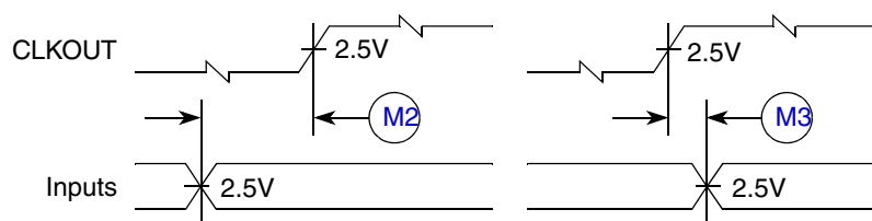
Figure A-2. General Purpose Input Timing Specifications
