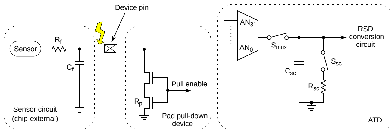
Figure 33-21. Predischarge Circuit
