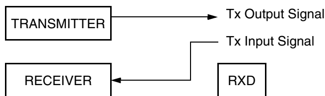
Figure 31-36. Single-Wire Operation (LOOPS = 1, RSRC = 1)
