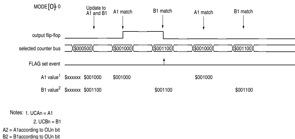
Figure 32-21. Double Action Output Compare with FLAG set on the second match
