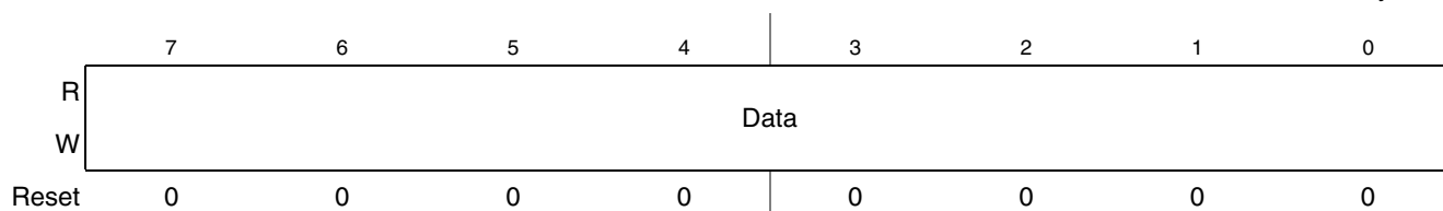
Figure 29-10. I 2 C Bus Data I/O Register (IBDR)
