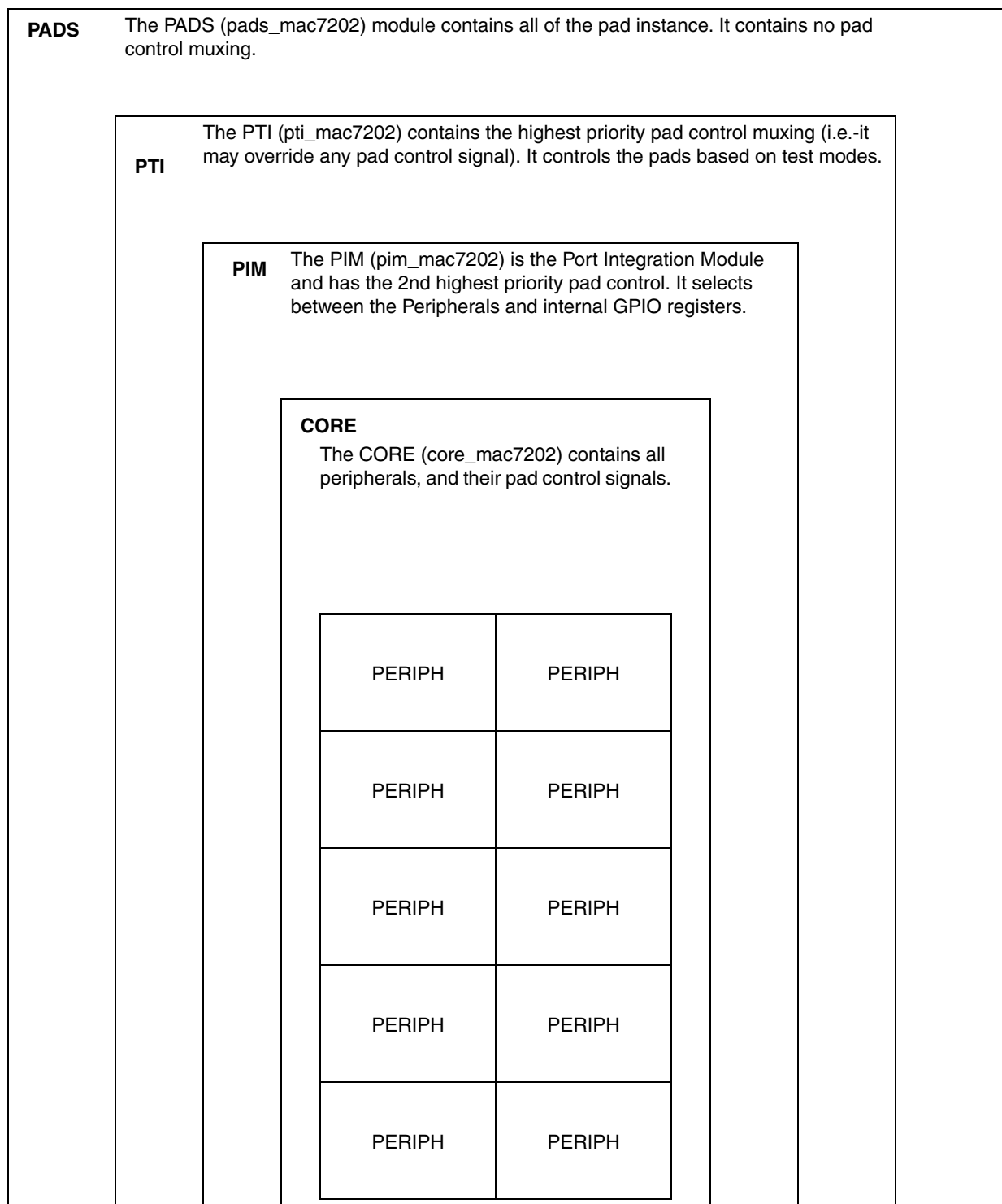
Figure 34-24. I/O Pad Control (Overview)
