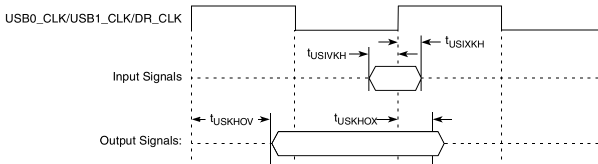
Figure 18. USB Signals
