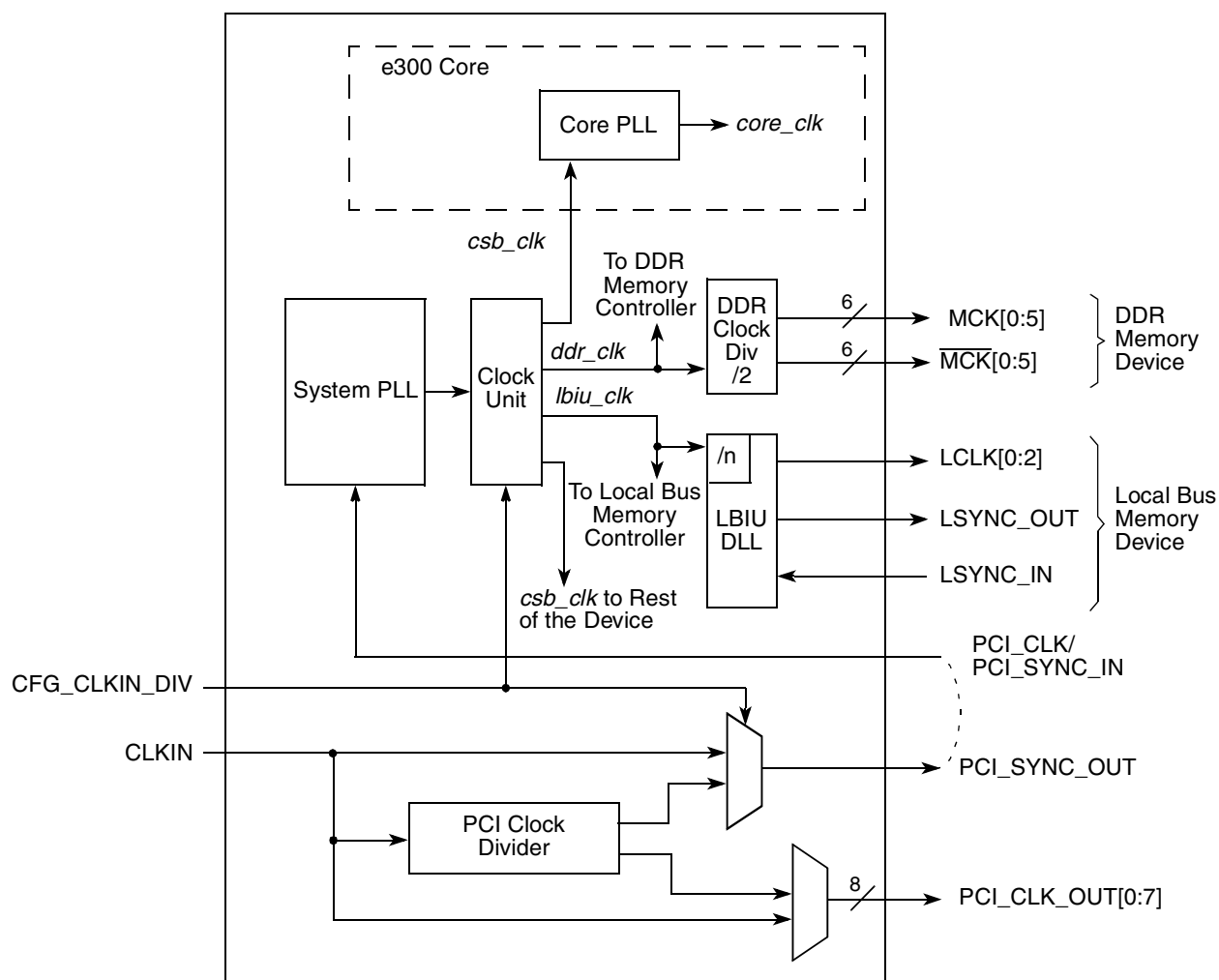
Figure 40. MPC8349EA Clock Subsystem
