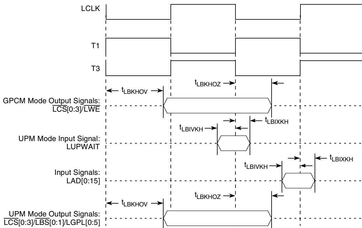
Figure 25. Local Bus Signals, GPCM/UPM Signals for LCCR[CLKDIV] = 2
