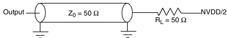
Figure 54. SPI AC Test Load
