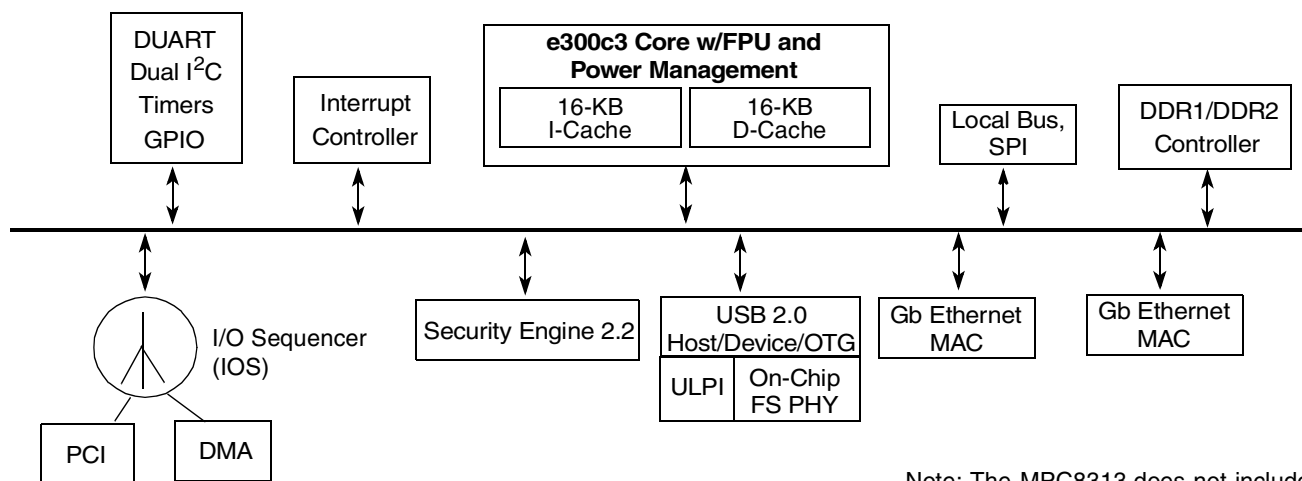
Figure 1. MPC8313E Block Diagram
