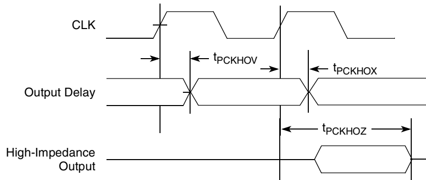
Figure 35. PCI Output AC Timing Measurement Condition
