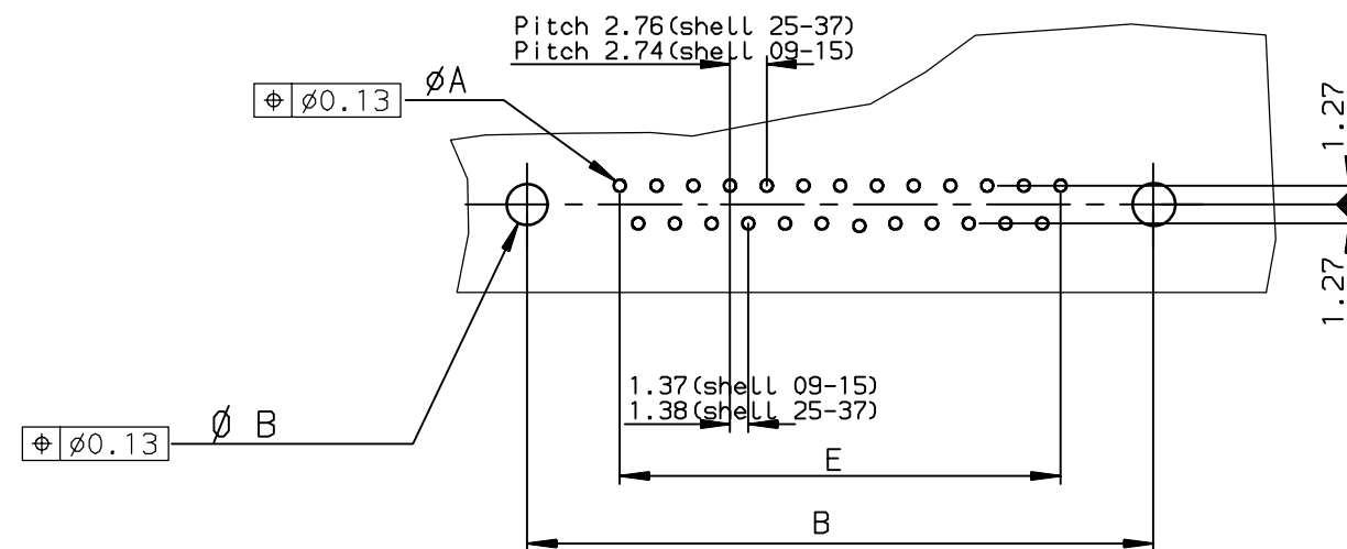
PC card drilling dimensions(after plating) (thickness 1.60 ±0.20 )
