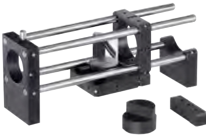
Mounting example of Corner connector 40, in front you can see the Corner connector 40 with thread
