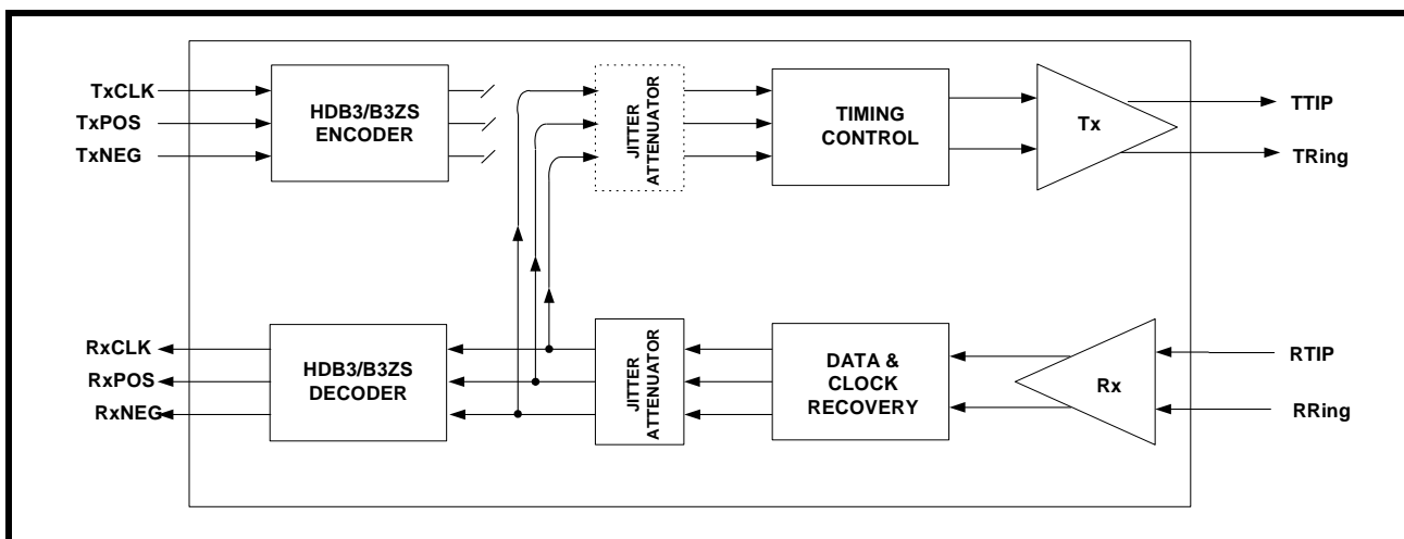
FIGURE 32. REMOTE LOOPBACK
