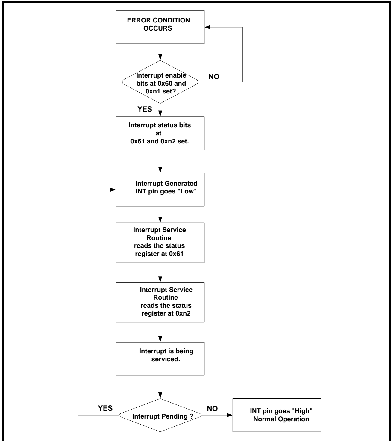
FIGURE 37. INTERRUPT PROCESS
