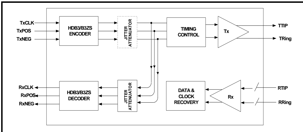
FIGURE 31. DIGITAL LOOPBACK
