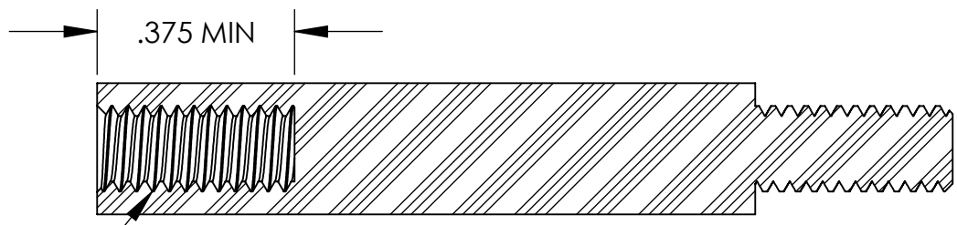
SECTION A-A 8-32 THREADS
