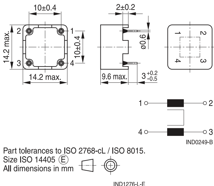
Horizontal version (B82720A)
