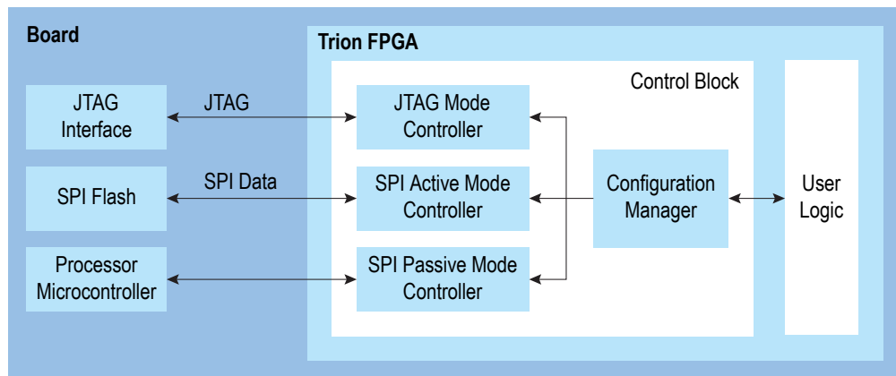
Figure 19: High-Level Configuration Options
