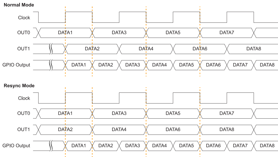
Figure 11: DDIO Output Timing Waveform
