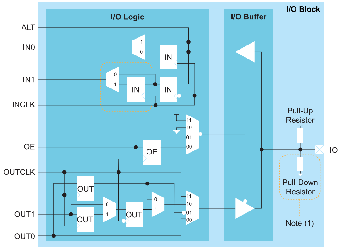
Figure 9: I/O Interface Block
