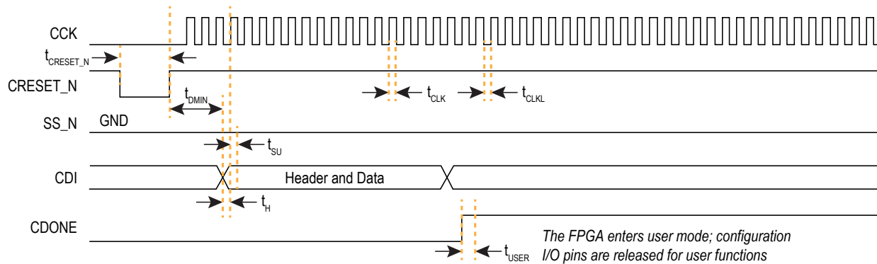
Figure 21: SPI Passive Mode (x1) Timing Sequence
