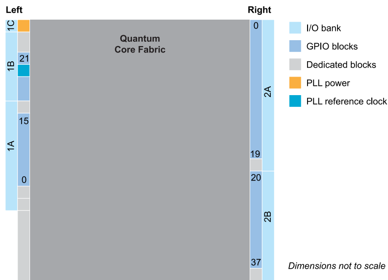
Figure 23: Floorplan Diagram for BGA49 and BGA81 Packages
