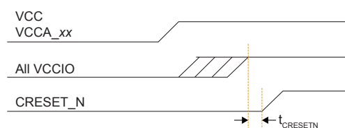
Figure 18: Trion ® FPGA Power Up Sequence
