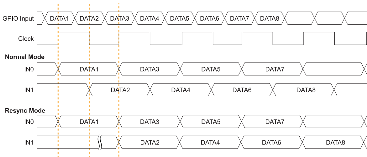
Figure 10: DDIO Input Timing Waveform
