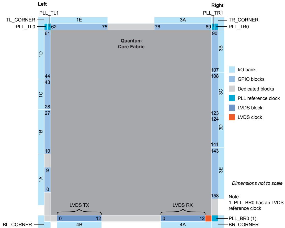
Figure 24: Floorplan Diagram for QFP144 Packages
