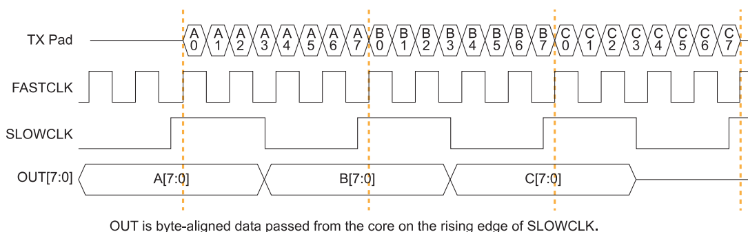
Figure 15: LVDS Timing Example Serialization Width of 8
