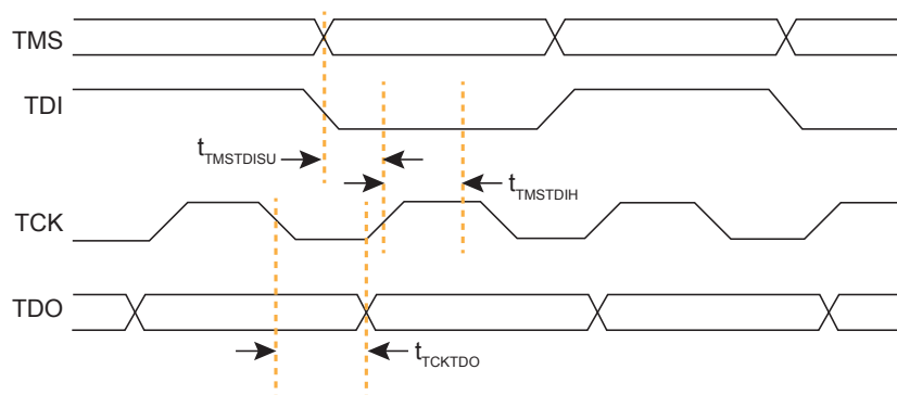
Figure 22: Boundary Scan Timing Waveform
