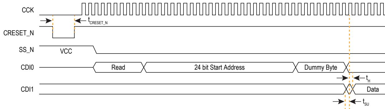
Figure 20: SPI Active Mode (x1) Timing Sequence
