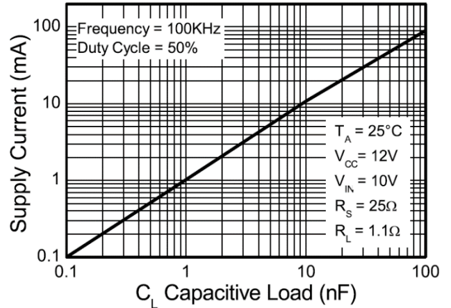
Supply Current
