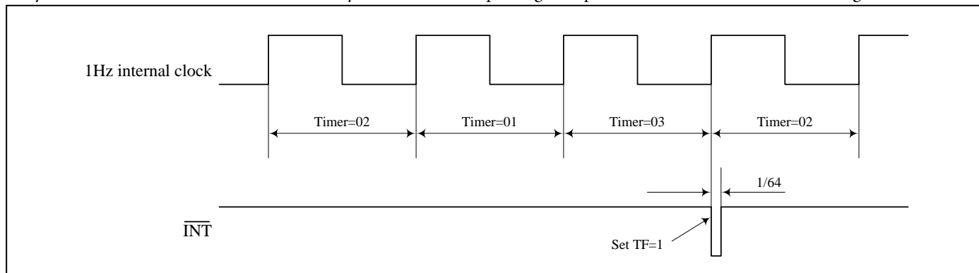
Fig.2 Example 2 of Timer Interrupts
