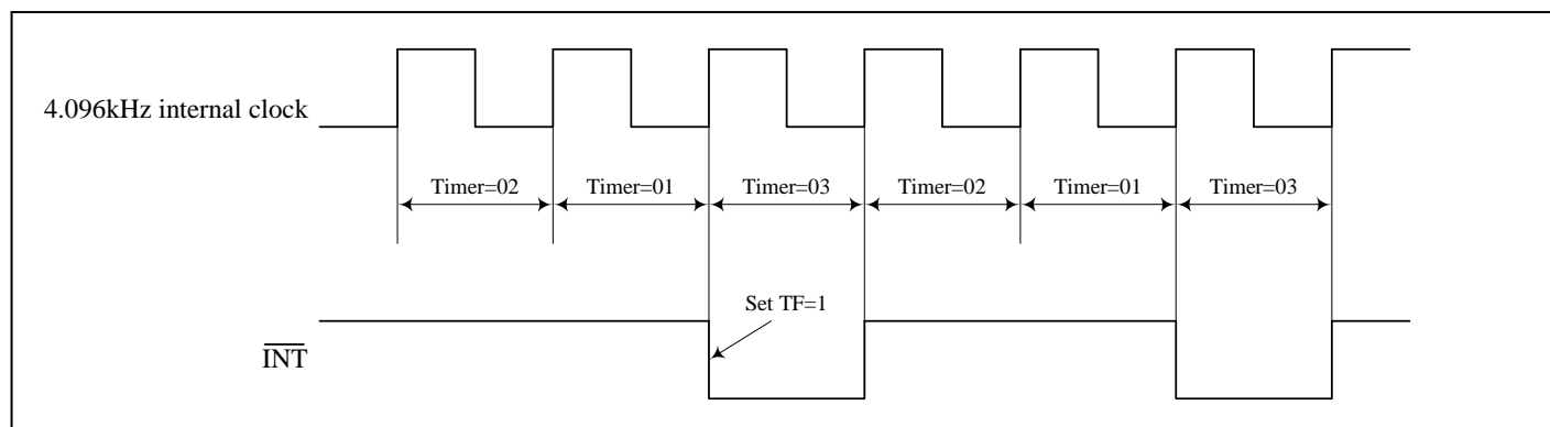
Fig.1 Example 1 of Timer Interrupts
