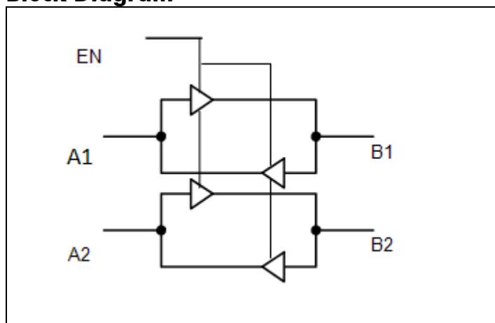
Figure 1: Block Diagram
