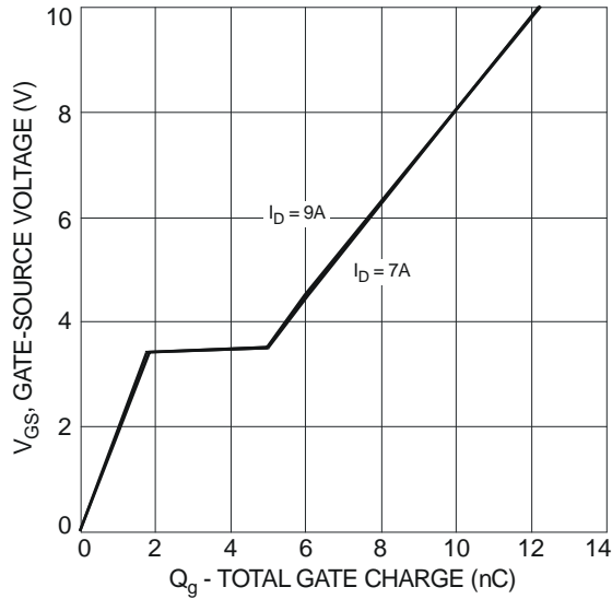
Fig. 7 Gate Charge
