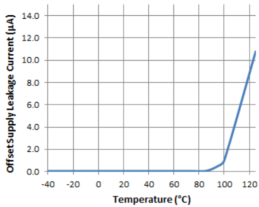
Figure 28. Offset Supply Leakage Current vs. Temperature
