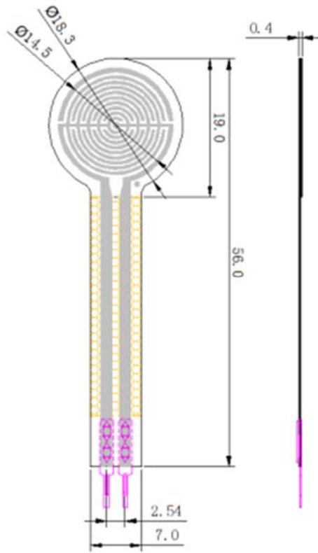
RP-C18.3-LT Dimension Diagram
