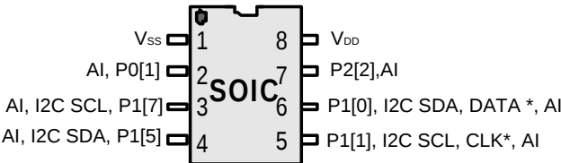
Figure 2. CY8C20134-12SXI 8-Pin SOIC Pinout
