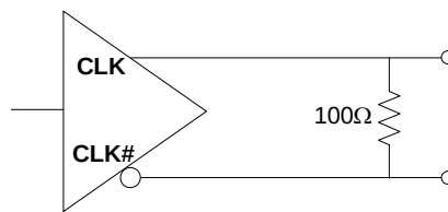
Figure 8. LVDS Termination
