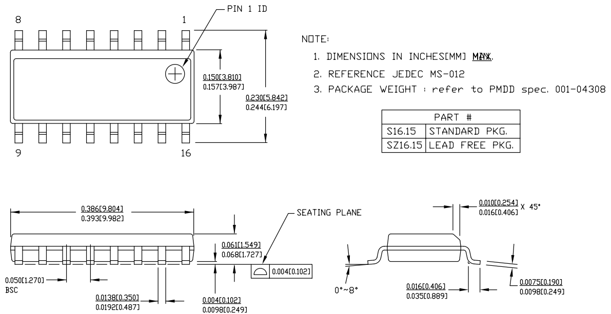
Figure 9. 16-pin SOIC (150 Mils)
