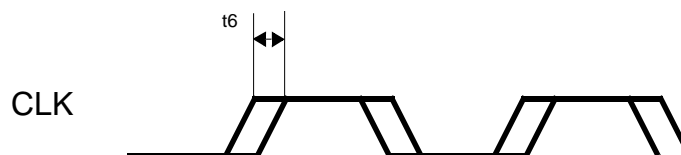
Figure 4. Peak-to-Peak Jitter
