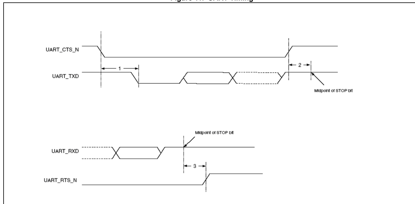
Figure 11. UART Timing
