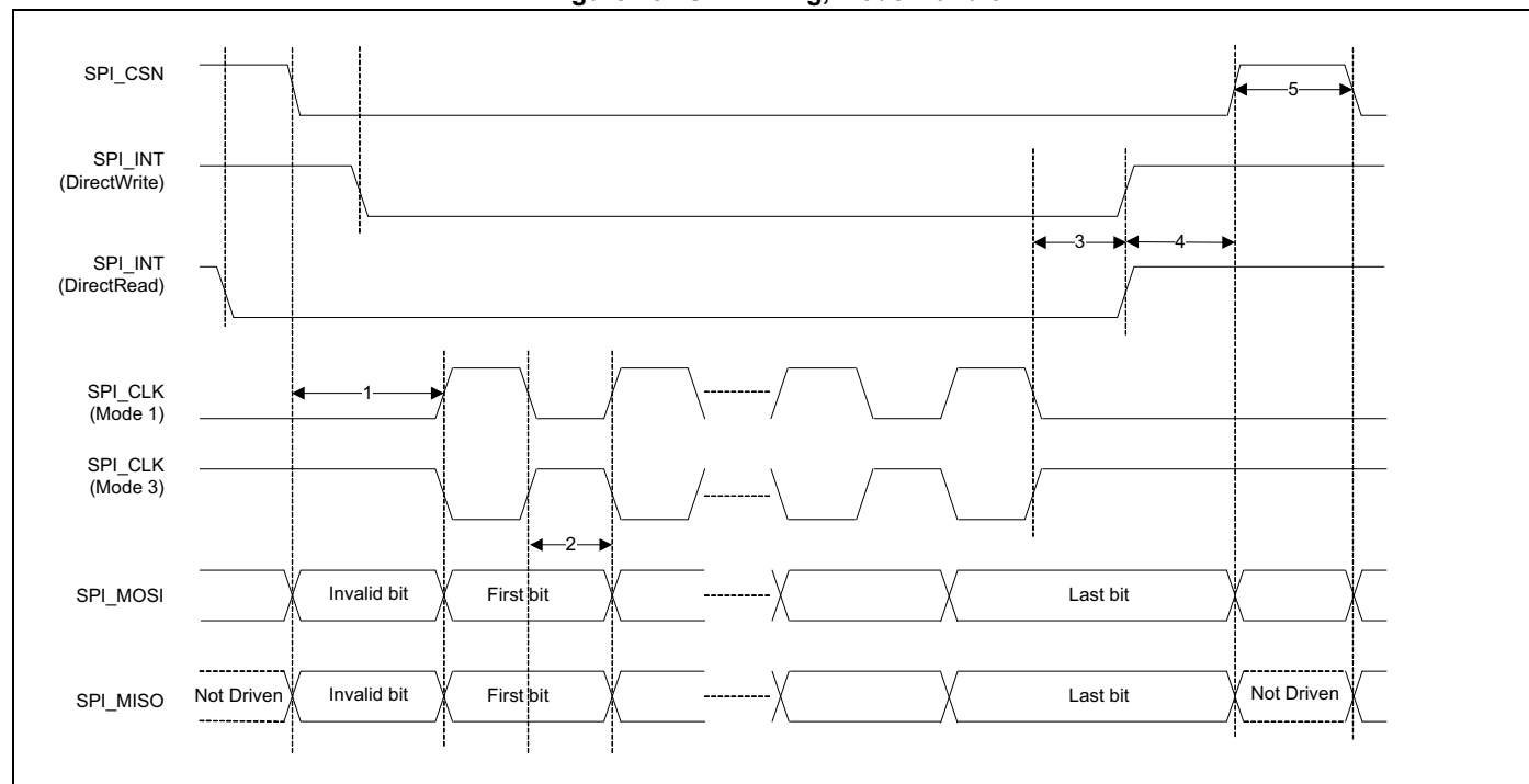
Figure 13. SPI Timing, Mode 1 and 3
