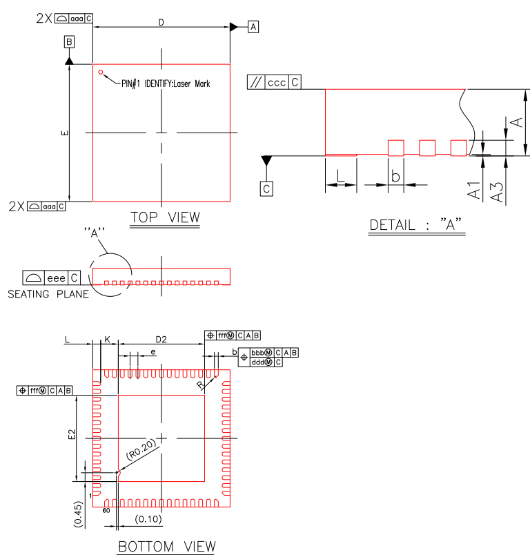
Figure 15. CYW20735 7 mm × 7 mm 60-Pin QFN Package
