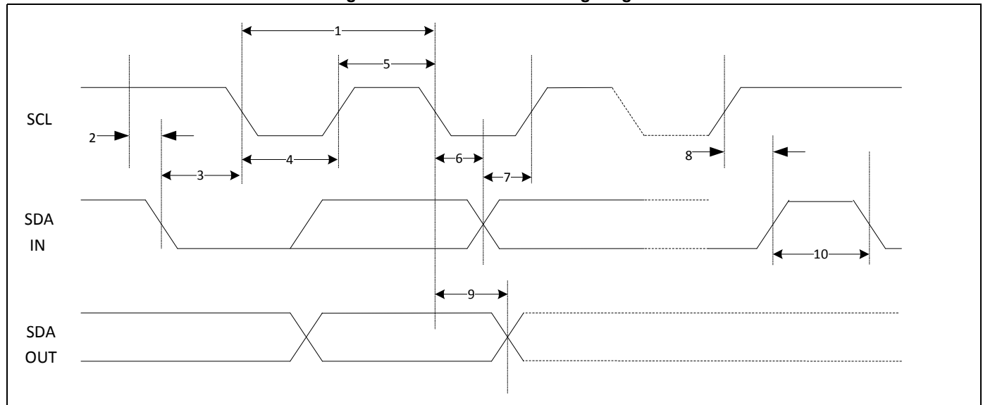
Figure 14. BSC Interface Timing Diagram
